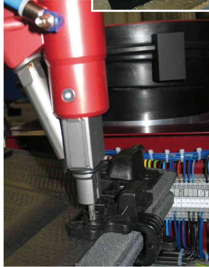
Luggage cover assembly
