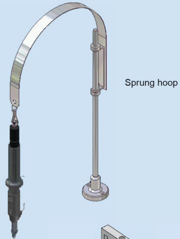
Parallelogram with pneumatic assistance
