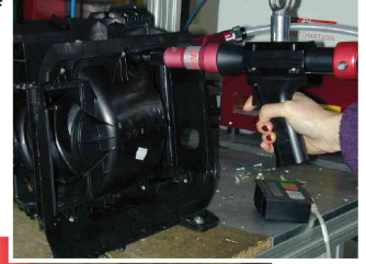
Horizontal assembly of air-conditioner units
